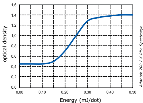
Dynamic Sensitivity
