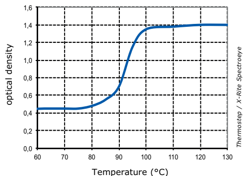
Static Sensitivity
